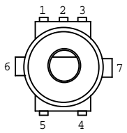
ROTARY SWITCH PINOUT ORIENTATION (FRONT VIEW)
